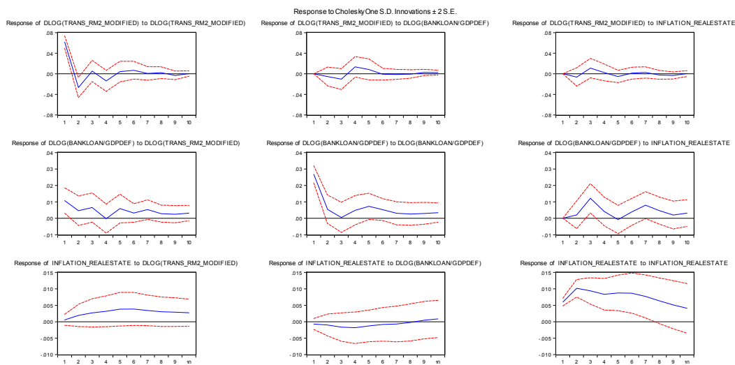
Figure 18 Impulse Response Functions, Model 3 d\log(\text{trans\_rm2\_modified}) d\log(\text{bankloan/gdpdef}) \text{inflation\_realestate} 1983q1 1995q4 Lag=4
